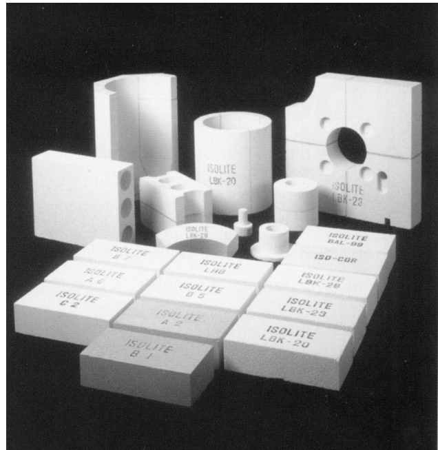
Fig.1 Insulating Firebrick
